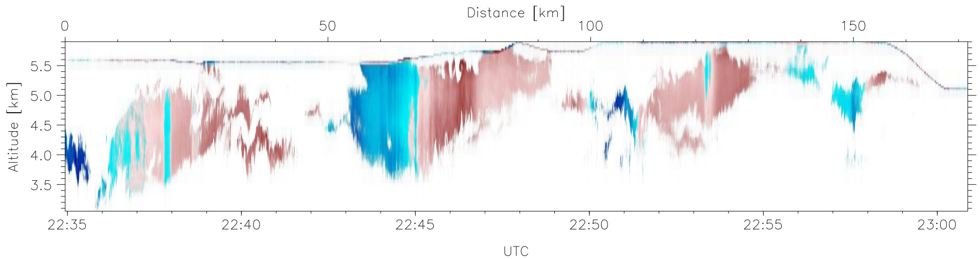
W2009-02-16-22-34-56: Down-slant Doppler
