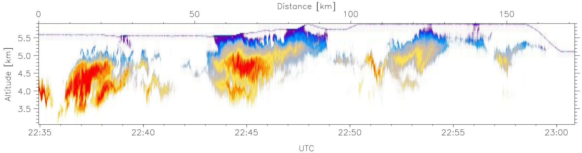
W2009-02-16-22-34-56: Down-slant Reflectivity
