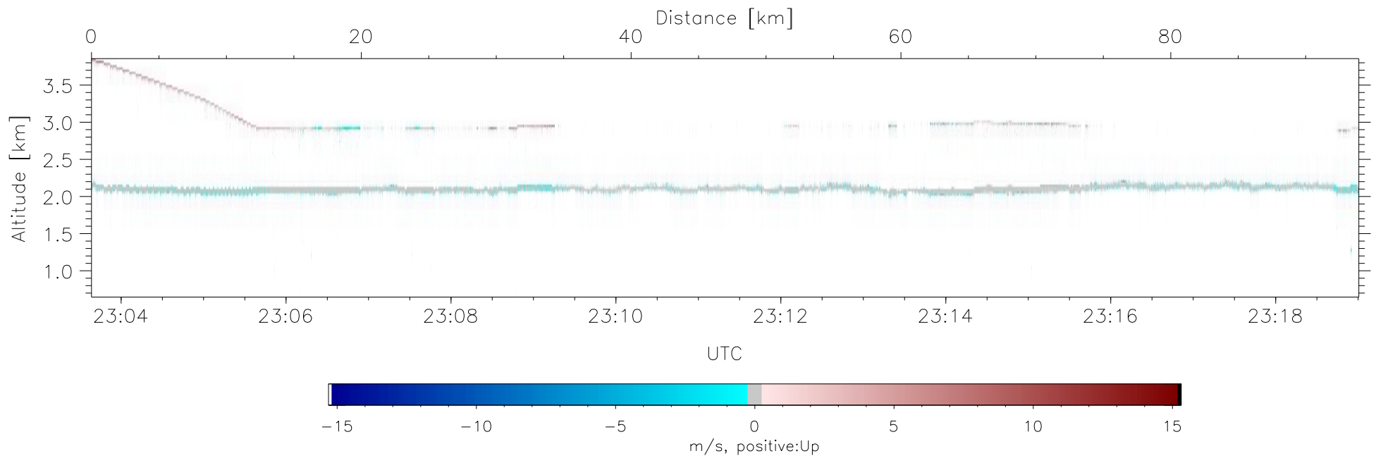
W2009-02-16-23-03-38, Up and Down Doppler, MaxVel Top/Bottom: 15.80/15.80
