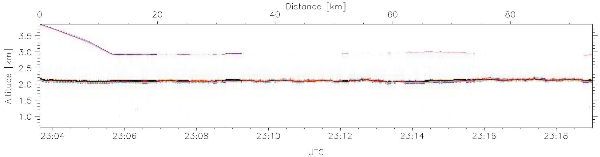
W2009-02-16-23-03-38, Up and Down Reflectivity
