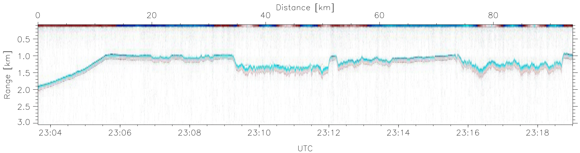
W2009-02-16-23-03-38: Down-slant Doppler
