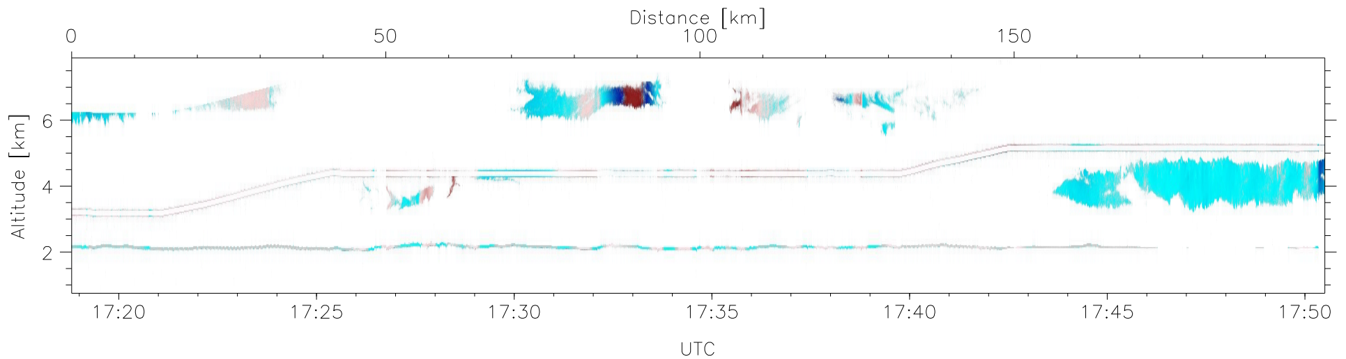
W2009-02-20-17-18-48, Up and Down Doppler, MaxVel Top/Bottom: 15.80/15.80
