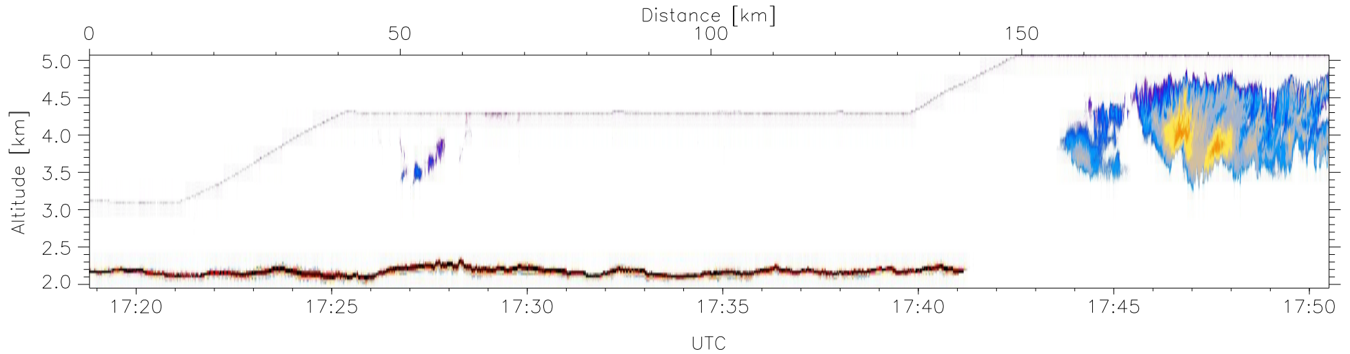
W2009-02-20-17-18-48: Down-slant Reflectivity
