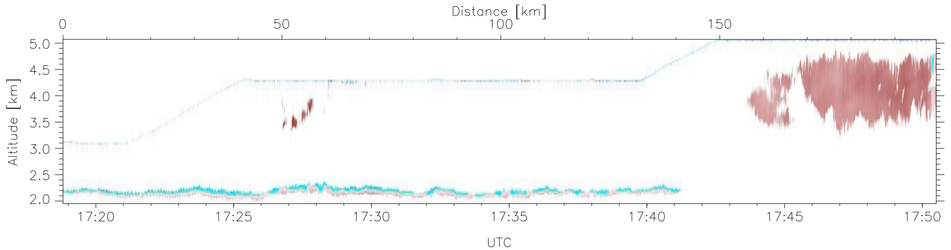
W2009-02-20-17-18-48: Down-slant Doppler
