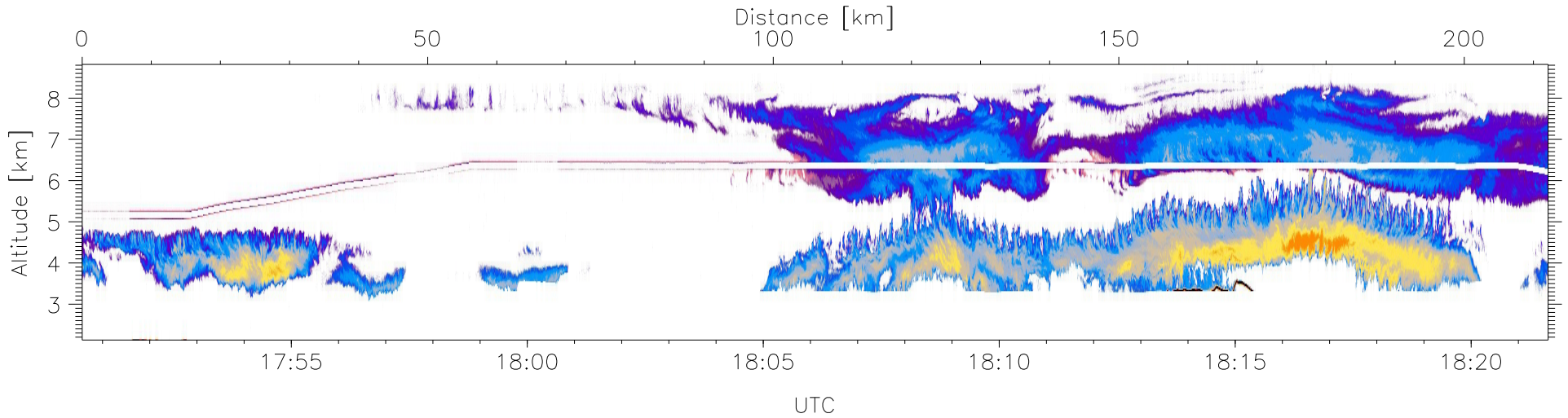
W2009-02-20-17-50-34, Up and Down Reflectivity
