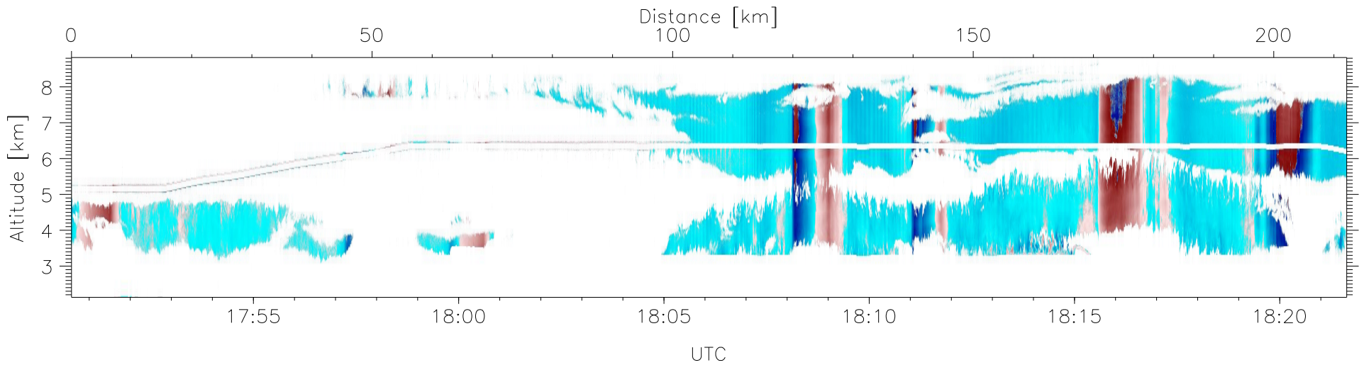
W2009-02-20-17-50-34, Up and Down Doppler, MaxVel Top/Bottom: 15.80/15.80
