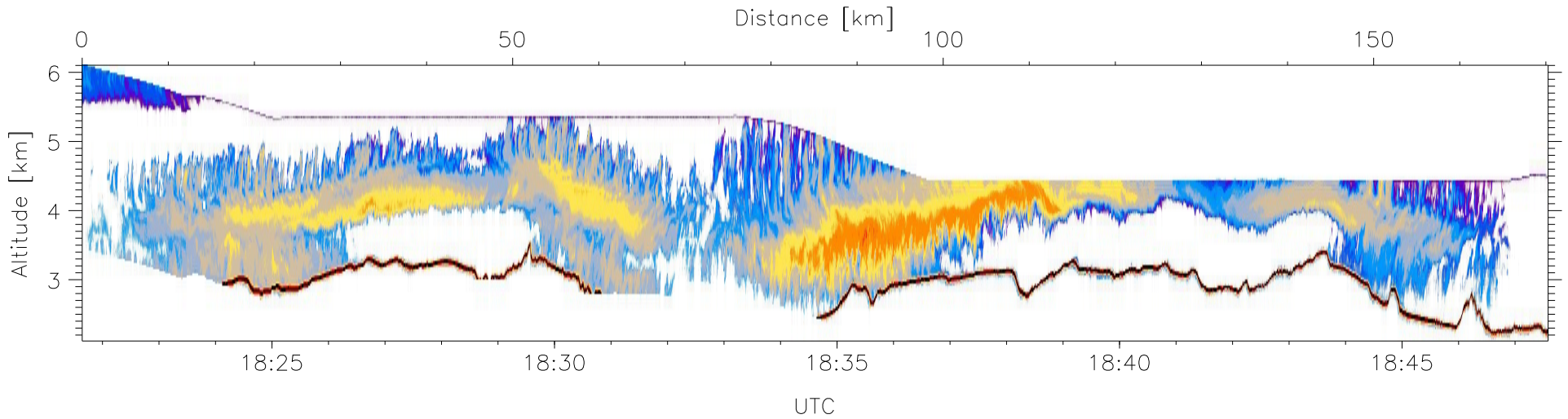
W2009-02-20-18-21-38: Down-slant Reflectivity
