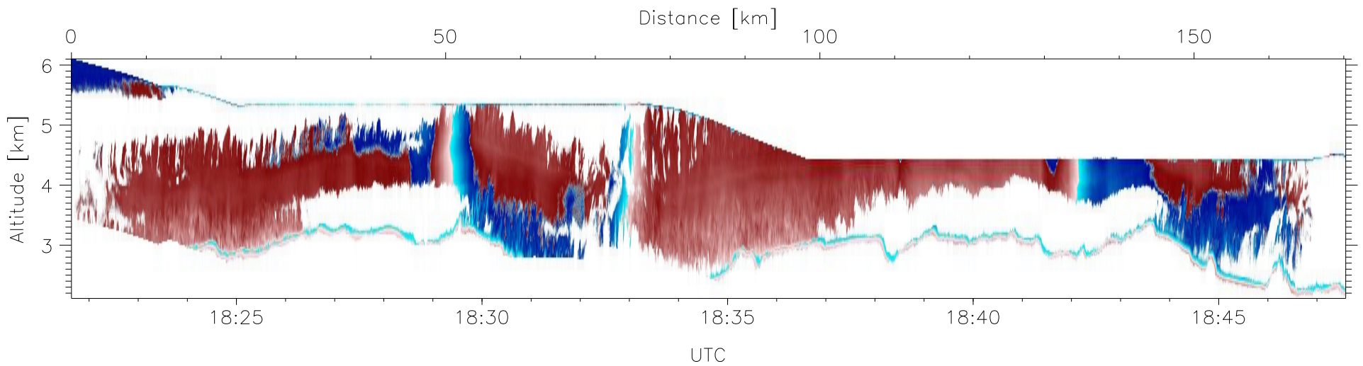
W2009-02-20-18-21-38: Down-slant Doppler
