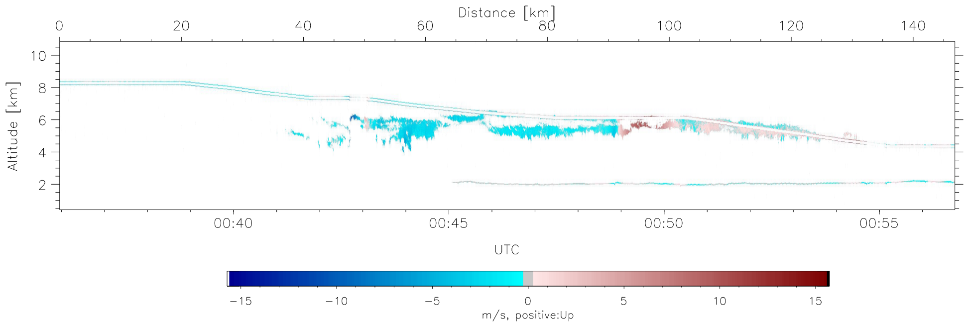
W2009-03-05-00-35-57, Up and Down Doppler, MaxVel Top/Bottom: 15.80/15.80
