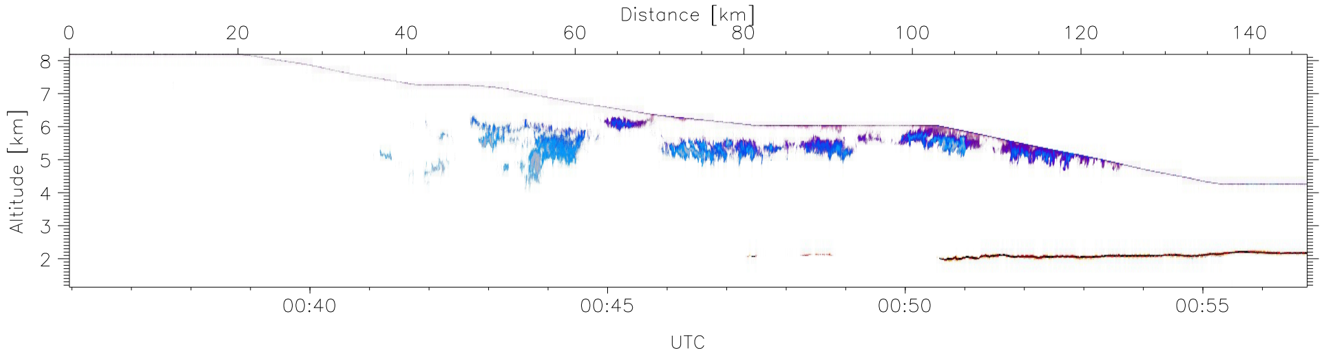
W2009-03-05-00-35-57: Down-slant Reflectivity
