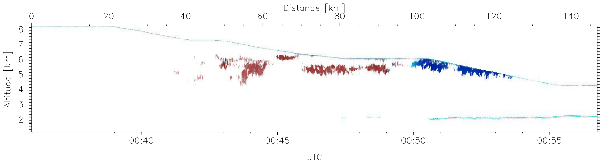
W2009-03-05-00-35-57: Down-slant Doppler
