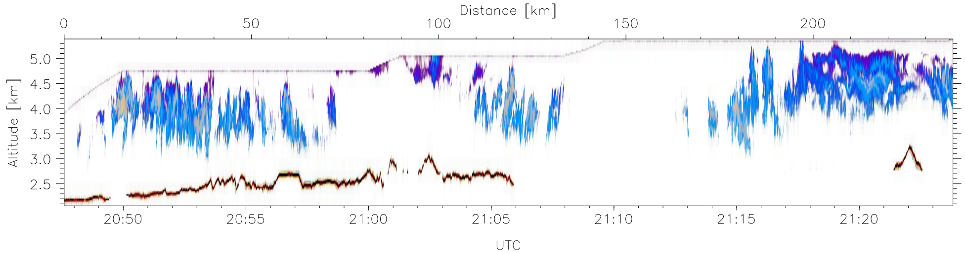
W2009-03-06-20-47-35: Down-slant Reflectivity
