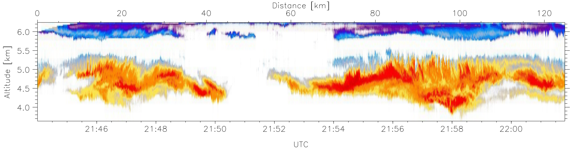
W2009-03-06-21-23-50: Down-slant Reflectivity
