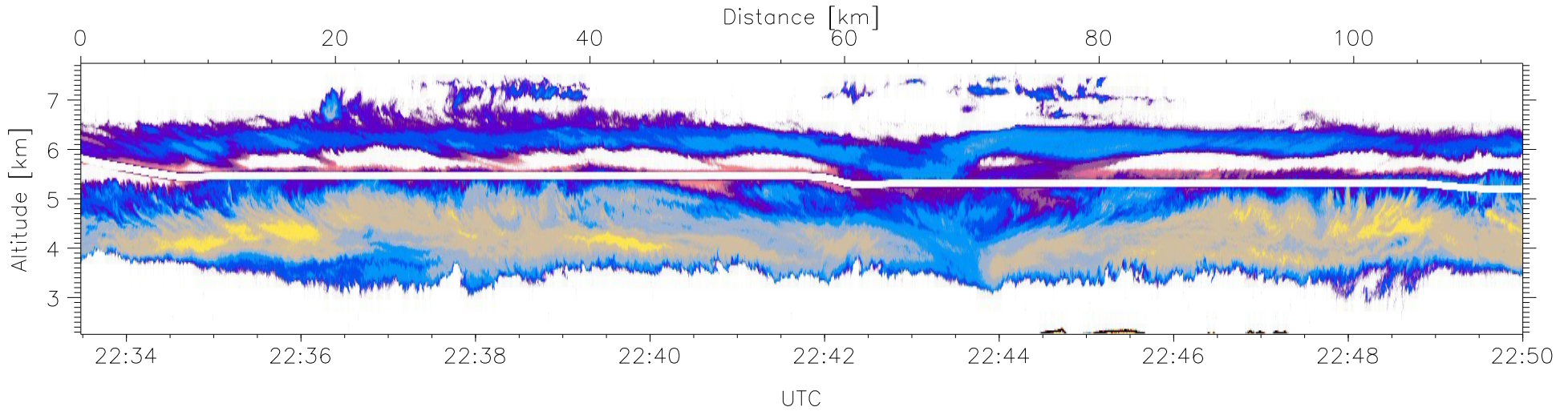
W2009-03-06-22-33-28, Up and Down Reflectivity
