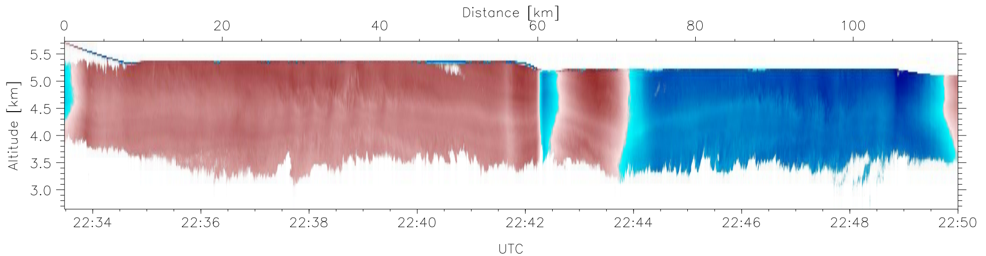
W2009-03-06-22-33-28: Down-slant Doppler
