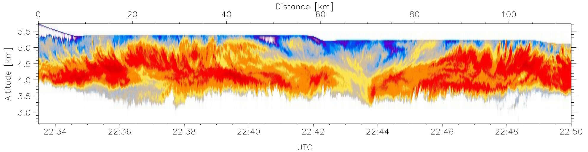
W2009-03-06-22-33-28: Down-slant Reflectivity
