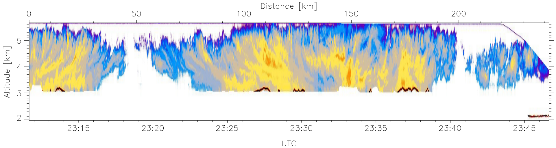
W2009-03-06-23-11-40: Down-slant Reflectivity
