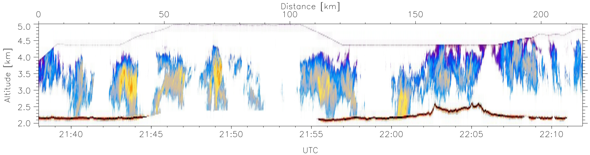
W2009-03-10-21-37-58: Down-slant Reflectivity
