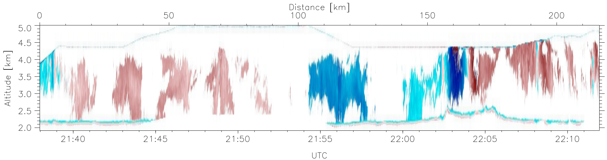
W2009-03-10-21-37-58: Down-slant Doppler
