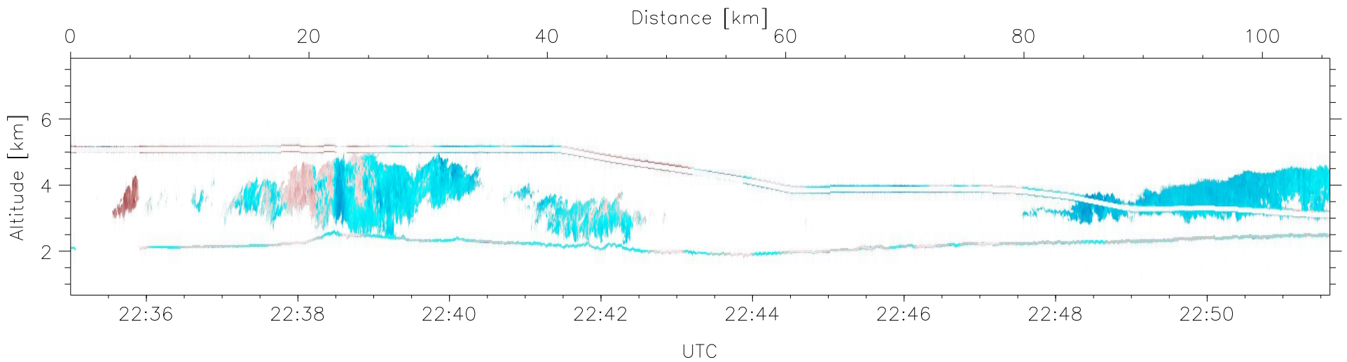
W2009-03-10-22-11-57, Up and Down Doppler, MaxVel Top/Bottom: 15.80/15.80
