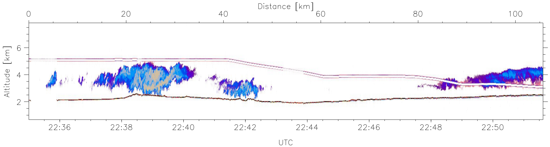
W2009-03-10-22-11-57, Up and Down Reflectivity
