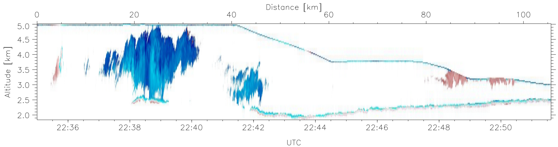
W2009-03-10-22-11-57: Down-slant Doppler
