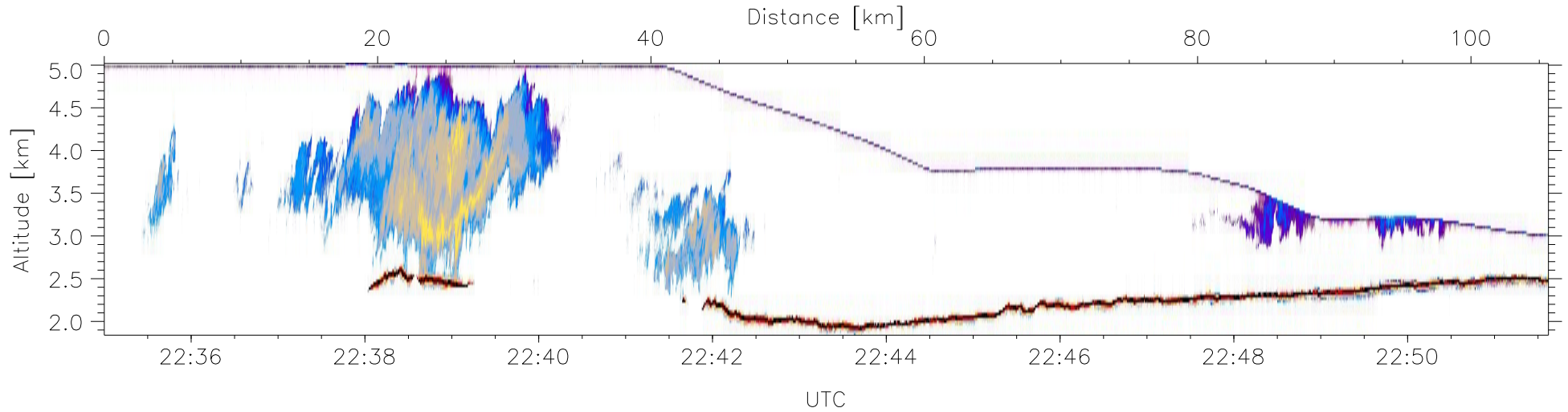
W2009-03-10-22-11-57: Down-slant Reflectivity
