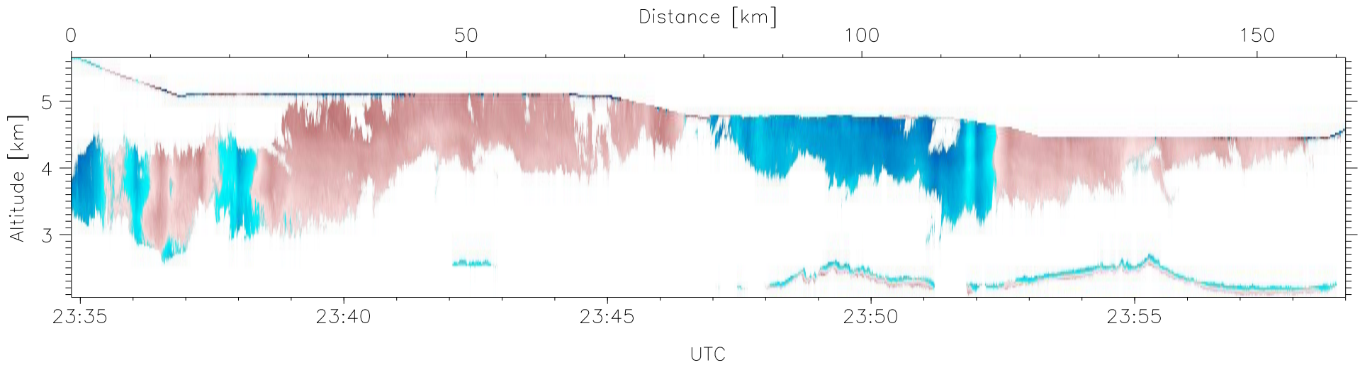
W2009-03-12-23-34-50: Down-slant Doppler
