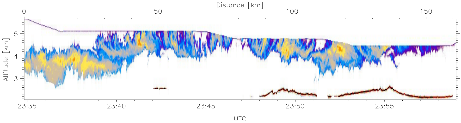
W2009-03-12-23-34-50: Down-slant Reflectivity
