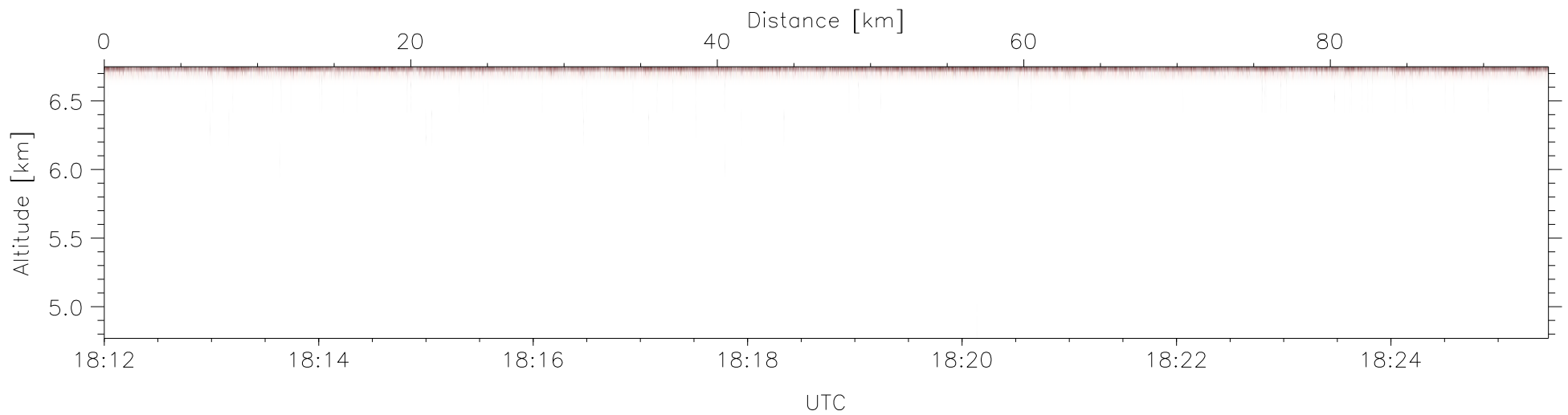
W2009-03-16-17-47-09: Down-slant Doppler
