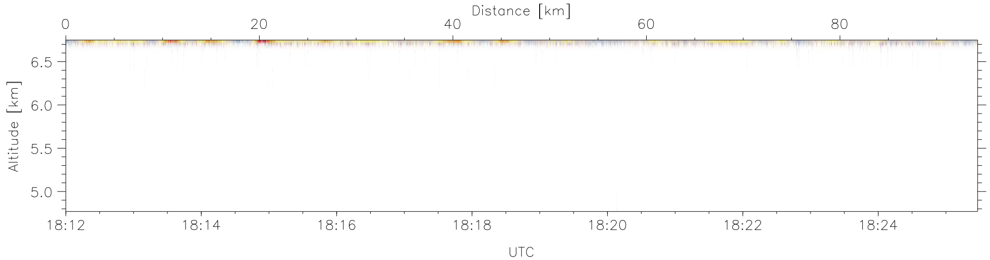
W2009-03-16-17-47-09: Down-slant Reflectivity
