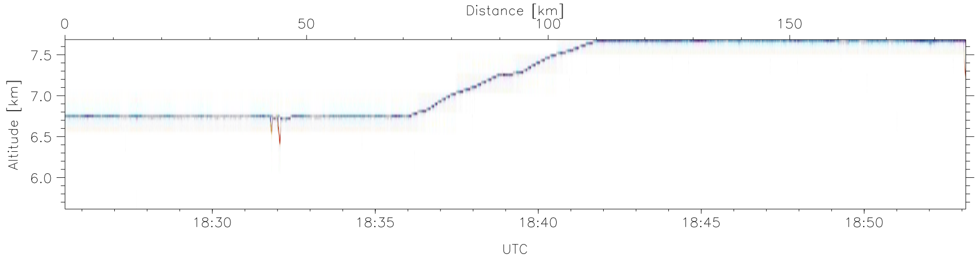
W2009-03-16-18-25-29: Down-slant Reflectivity
