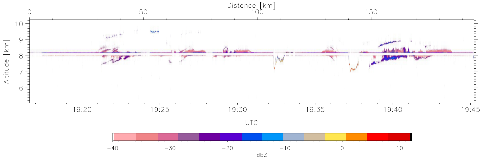
W2009-03-16-19-16-37, Up and Down Doppler, MaxVel Top/Bottom: 15.80/15.80
