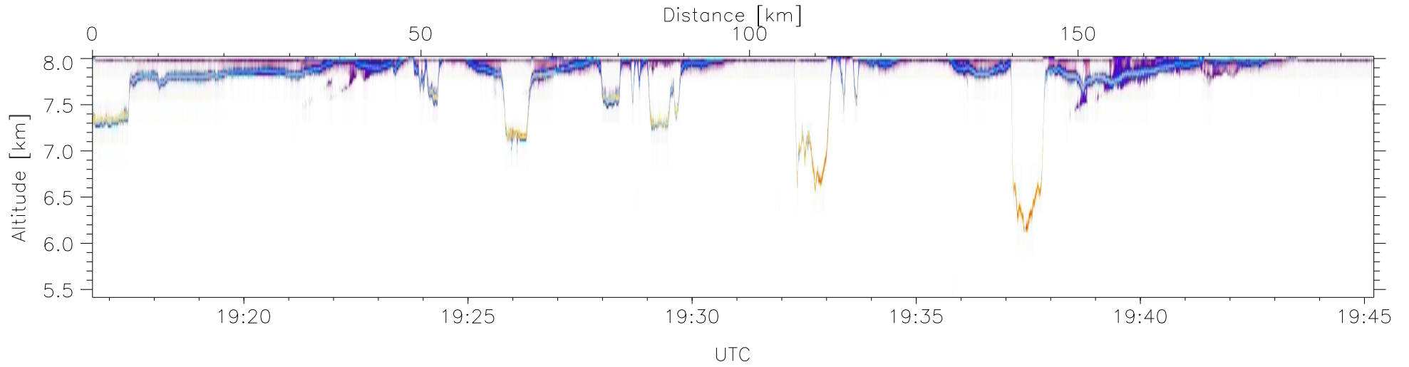
W2009-03-16-19-16-37: Down-slant Reflectivity
