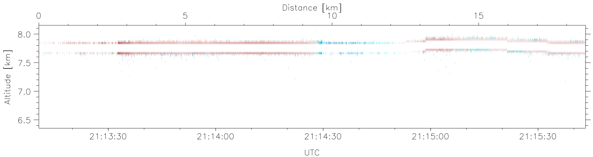
W2009-03-16-21-13-10, Up and Down Doppler
