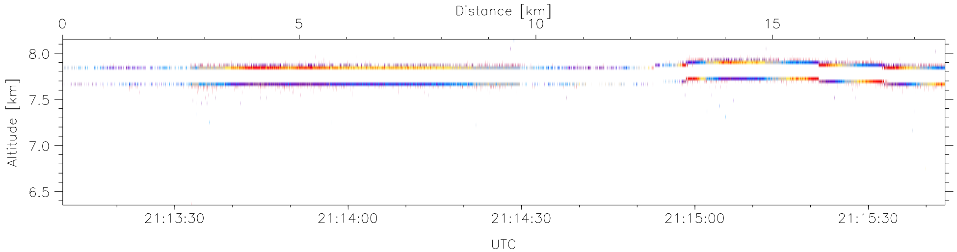
W2009-03-16-21-13-10, Up and Down Reflectivity
