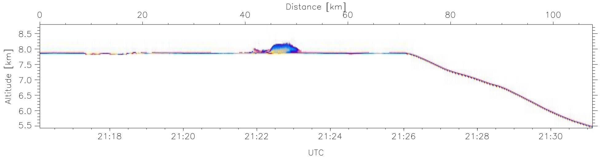
W2009-03-16-21-16-05: Up Reflectivity
