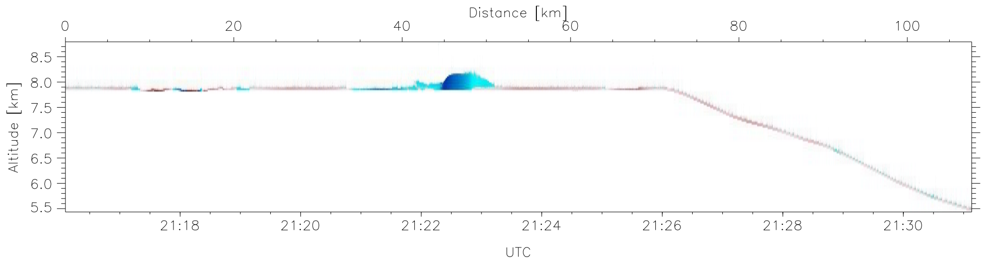
W2009-03-16-21-16-05: Up Doppler
