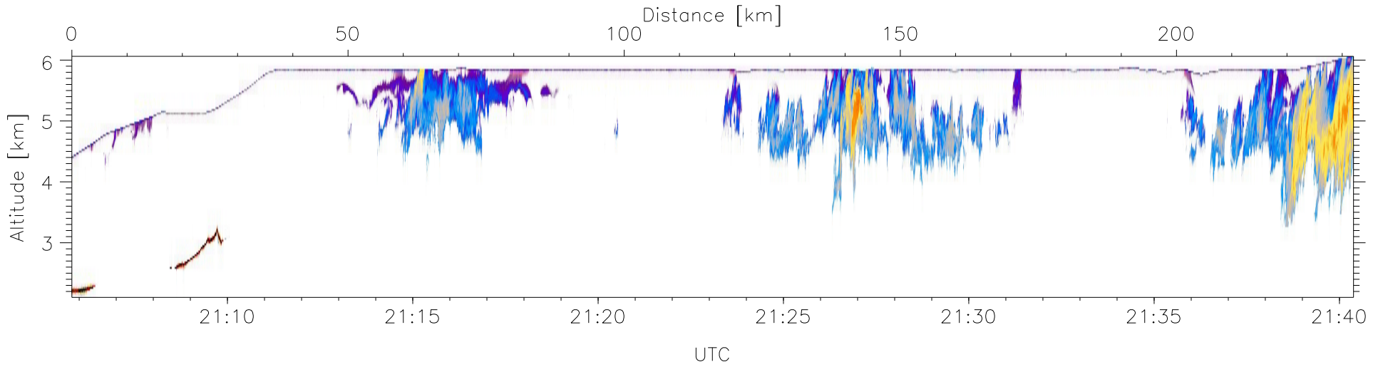
W2009-03-18-21-05-48: Down-slant Reflectivity
