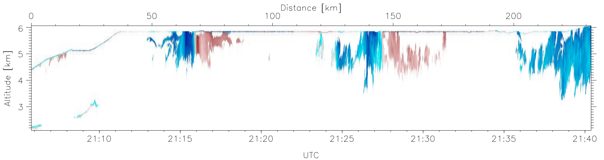
W2009-03-18-21-05-48: Down-slant Doppler
