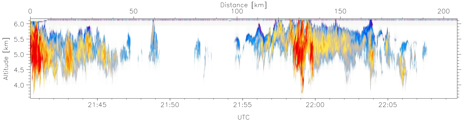
W2009-03-18-21-40-23: Down-slant Reflectivity
