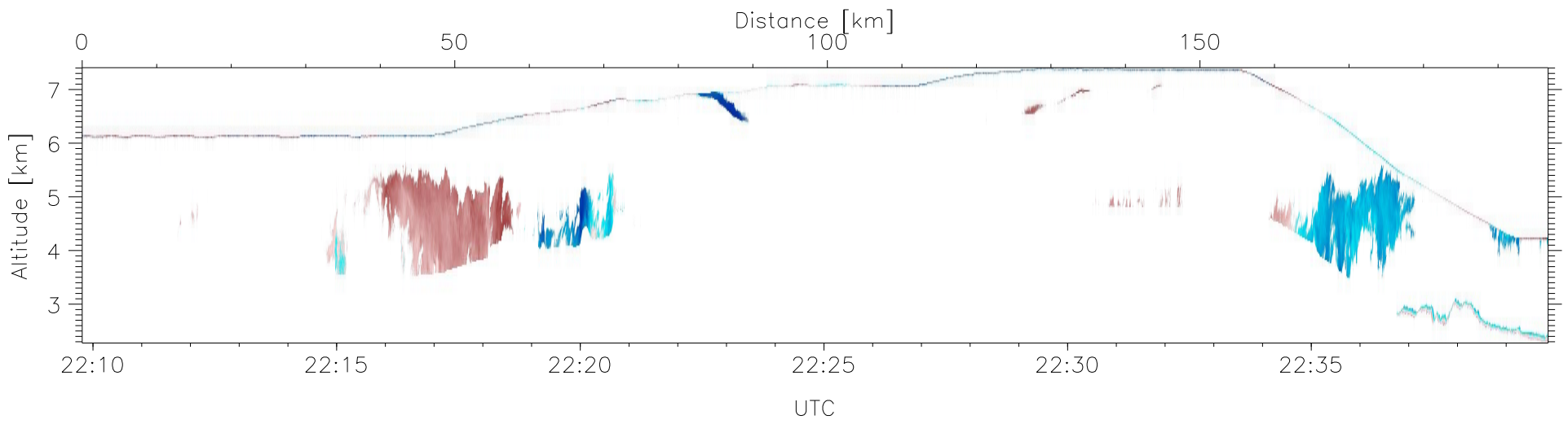
W2009-03-18-22-09-46: Down-slant Doppler
