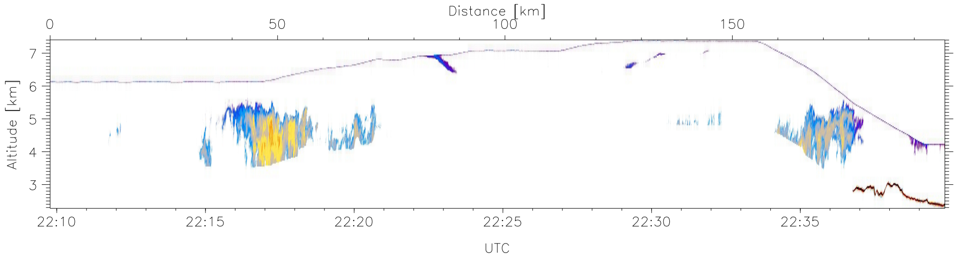
W2009-03-18-22-09-46: Down-slant Reflectivity
