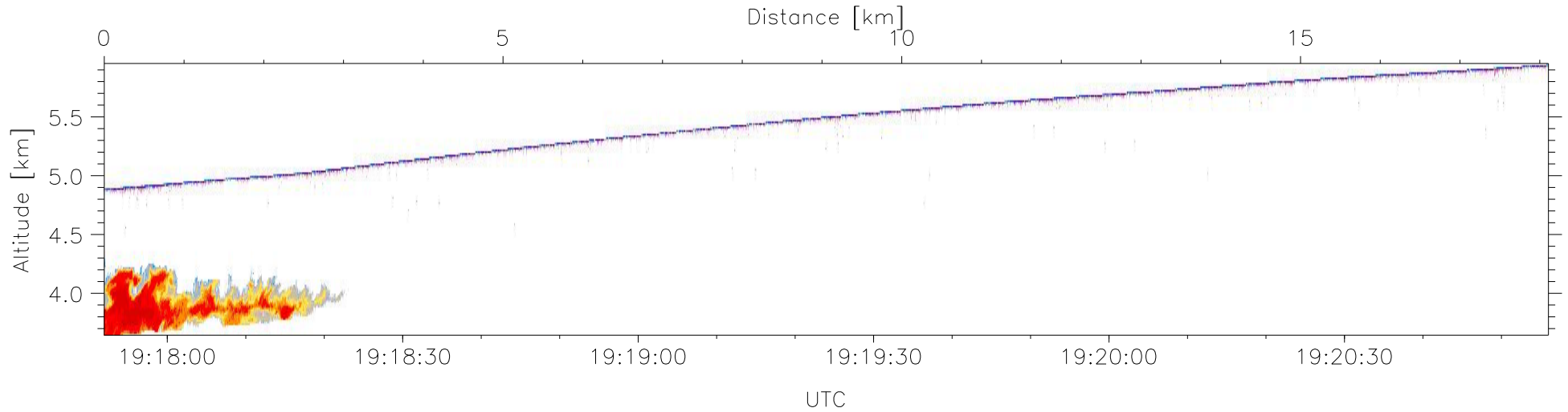
W2009-03-27-19-17-52: Down-slant Reflectivity
