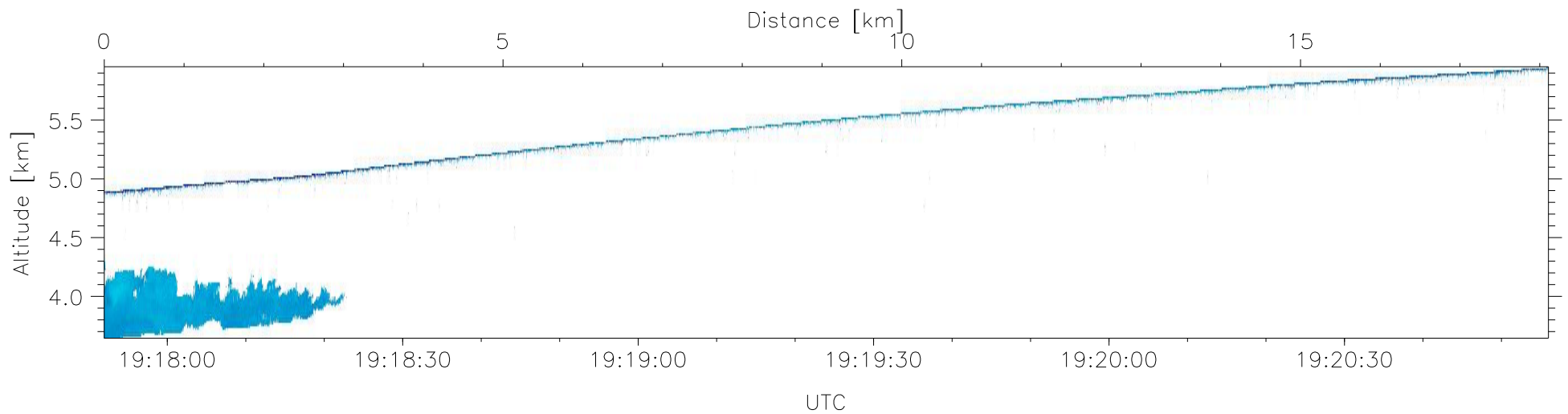
W2009-03-27-19-17-52: Down-slant Doppler
