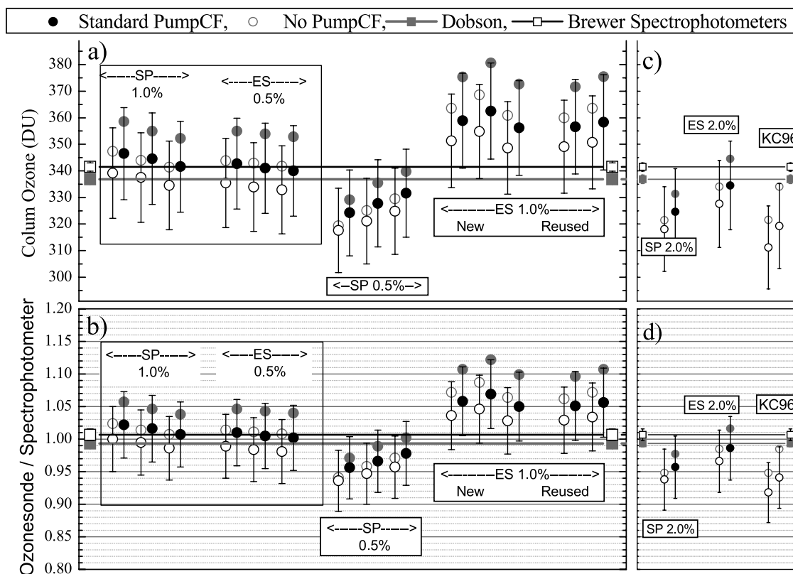
Figure 9. (a) Integrated ozone from the 12 core ozonesondes (3 SP1.0, 3 ES0.5, 3 SP0.5, and 3 ES1.0), two reused ES1.0 ozonesondes (circles with error bars), and from Dobson and Brewer spectrophotometers located at the launch site (lines with boxes and error bars). The ozonesonde measurements are extrapolated using both the SBUV climatology (40 DU for April at 41°N) (solid and open black circles) [McPeters et al. , 1997] and at constant ozone mixing ratio above the last ozone measurement (solid and open gray circles without error bars). Results with and without the standard pump efficiency correction [Komhyr, 1986] for measurements at low air pressures are shown. The error bars indicate a precision of 5%. The standard deviation of the seven Dobson and Brewer spectrophotometer measurements completed during the balloon flight do not exceed the symbol sizes. (b) As in Figure 9a but ratios of integrated total ozone from the ozonesondes to the average of the Dobson and Brewer measurements. (c and d) Same as Figures 9a and 9b for the other four auxiliary ozonesondes flown (1 SP2.0, 1 ES2.0, and 2 KC96). Results from the manufacturer's recommendations for solution strength are enclosed in the box in Figures 9a and 9b.
