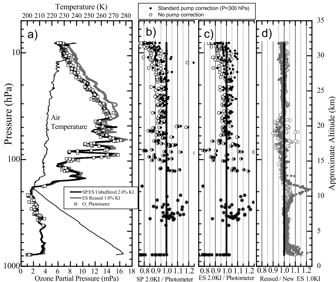
Figure 6. Profiles of (a) air temperature and ozone partial pressure from the ozone photometer, one SP2.0 and one ES2.0 ozonesonde, and 2 reused ES1.0 ozonesondes; (b) ratios of SP2.0 to photometer with and without a pump correction; (c) ratios of ES2.0 to photometer with and without a pump correction; and (d) ratios of the two reused ES1.0 measurements (open and solid gray circles) to the average of the three new ES1.0 ozonesondes. For the ozonesonde partial pressure profile the measurements were corrected for pump efficiency at air pressures less than 300 hPa, using Komhyr [1986].
