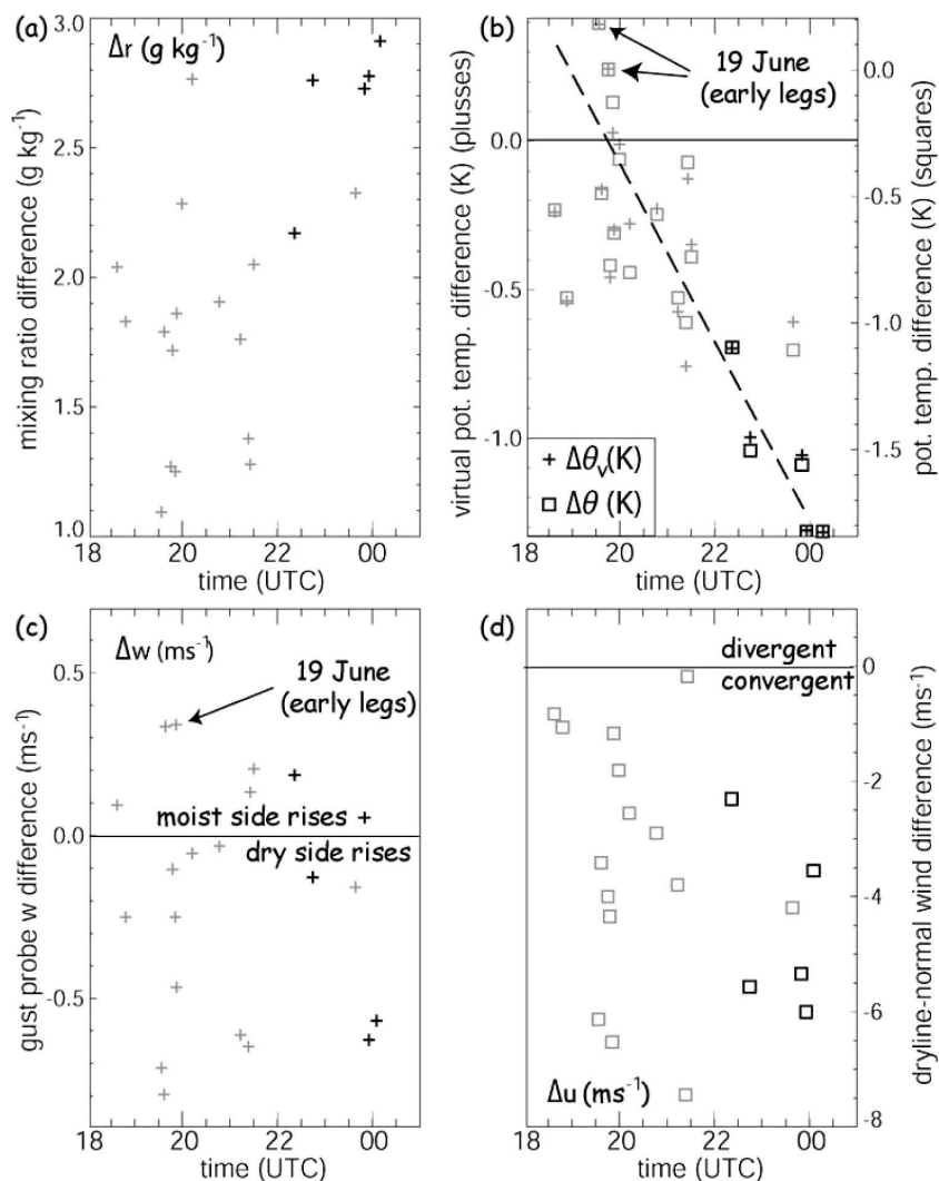
FIG. 13. Temporal change of the difference between moist and dry air, based on in situ WKA data at low flight levels (below 0.5h_{ac} ), for all dryline cases in this study (five legs on 22 May, three on 24 May, nine for 18 Jun, and four for 19 Jun). The difference (moist – dry) is based on 3-km averages, on opposite sides of the dryline moisture gradient. Black symbols apply to 22 May, gray symbols to the other days. The dashed line in (b) is the linear best fit for \theta_v .
