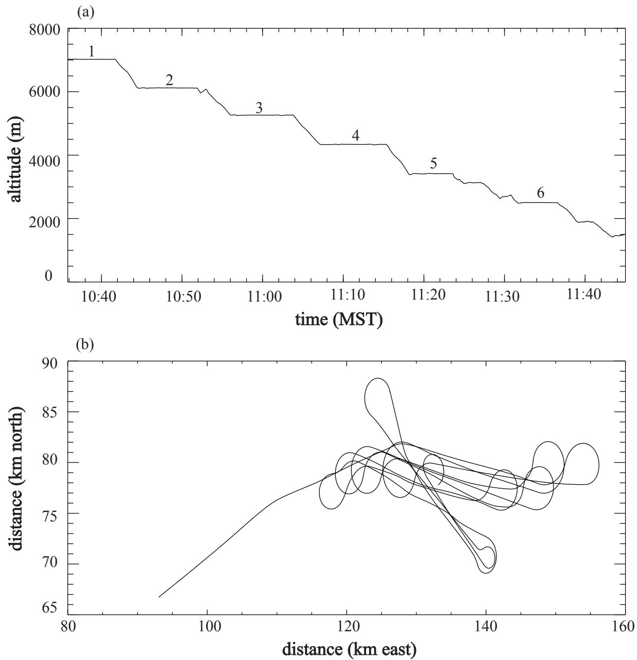
Fig. 1. (a) Time series of aircraft altitude (b) flight track horizontal projection for October 31 1992.
