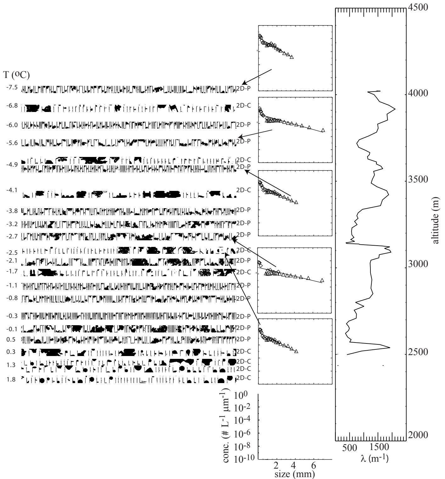
Fig. 11. Sample 2D images during the spiral descent on September 06, 1995. The middle panel shows sample particle spectra. The best exponential fit for the spectra is also drawn. The scale for the spectral plots are shown the bottom. The right-most panel shows corresponding \lambda values of the spectra as defined in the text.
