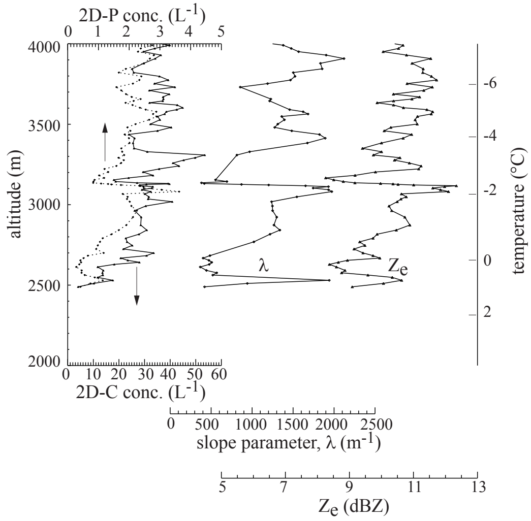
Fig. 14. Vertical profiles of particle concentrations, slope parameter, \lambda , and equivalent reflectivity factor, Z_e , during the spiral descent on Sept. 6, 1995.
