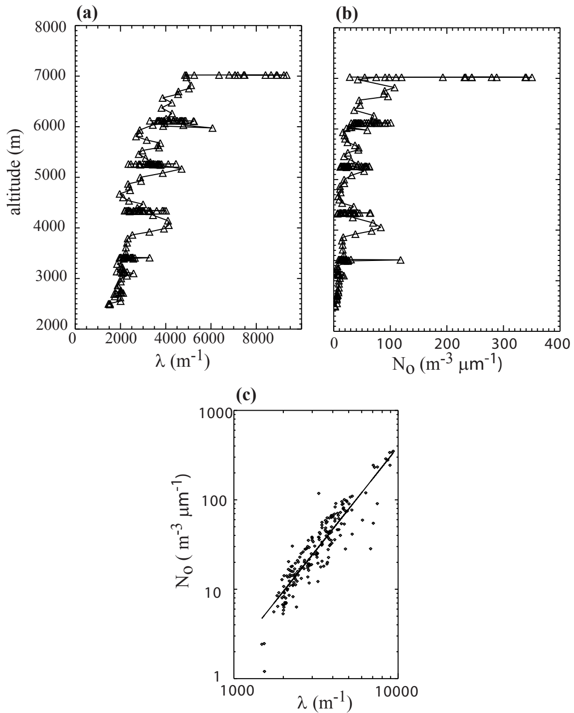
Fig. 6. Vertical profiles of (a) the slope parameter, \lambda , and (b) intercept parameter, N_0 for exponential fits to ice crystal size spectra, and (c) a scatter plot of \lambda versus N_0 during the staircase descent of October 31, 1992.
